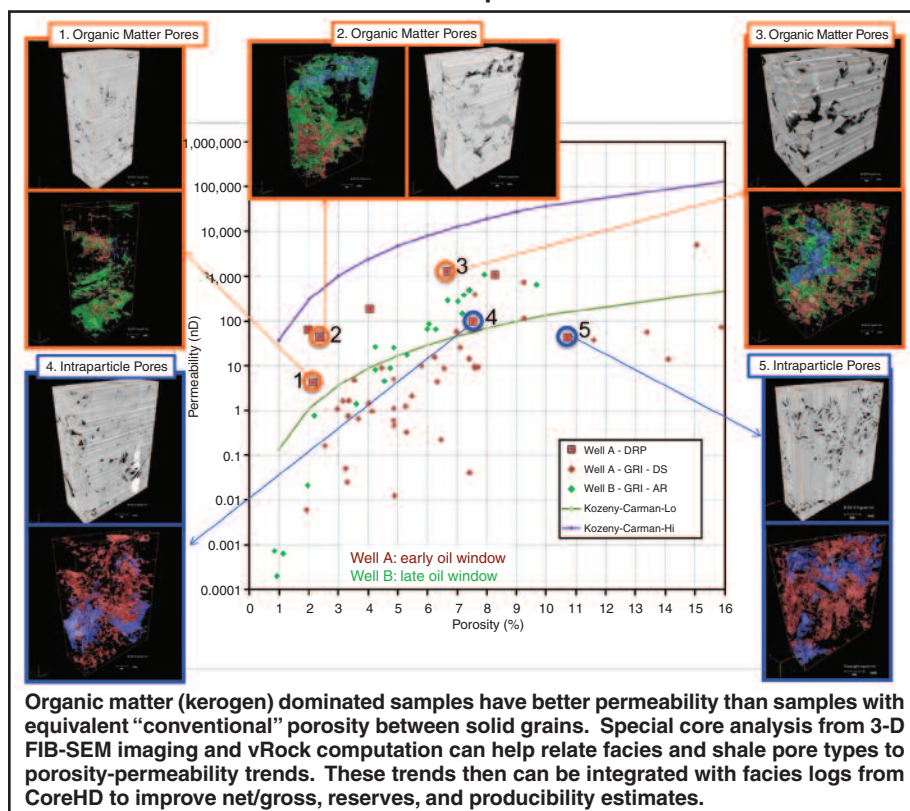
FIGURE 3 Special Core Analysis from 3-D FIB-SEM Imaging and vRock Computation
